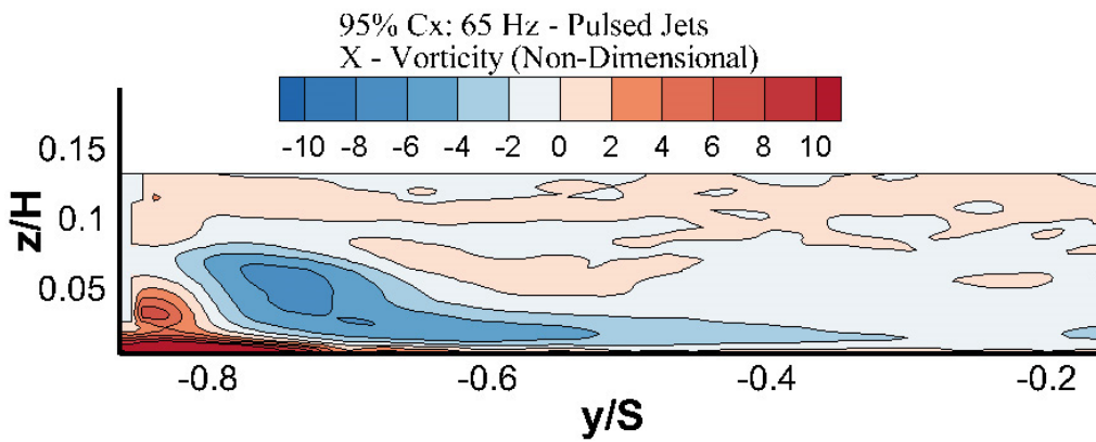
Figure 209. x – Vorticity - 65 Hz Pulsed Jets 95% Cx
