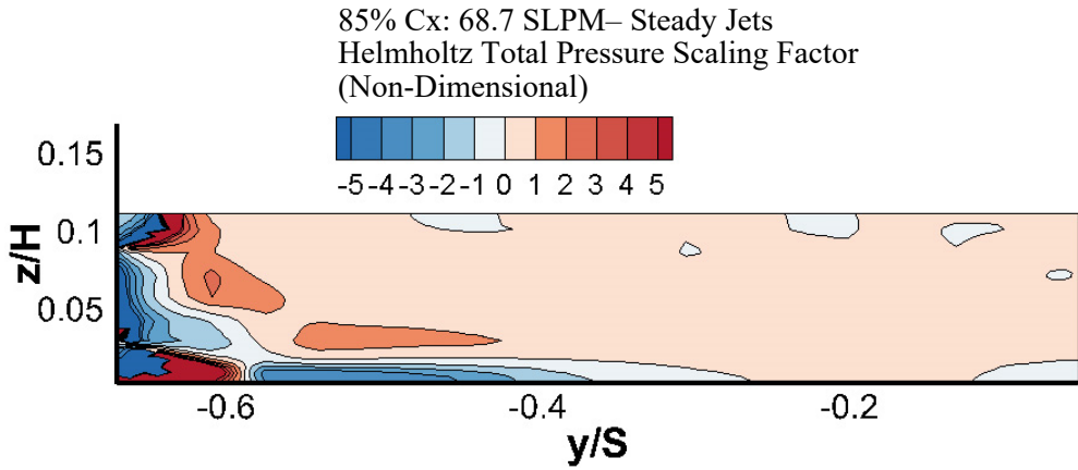
Figure 196. Helmholtz Total Pressure Scaling Factor - 68.7 SLPM Steady Jets 85%
