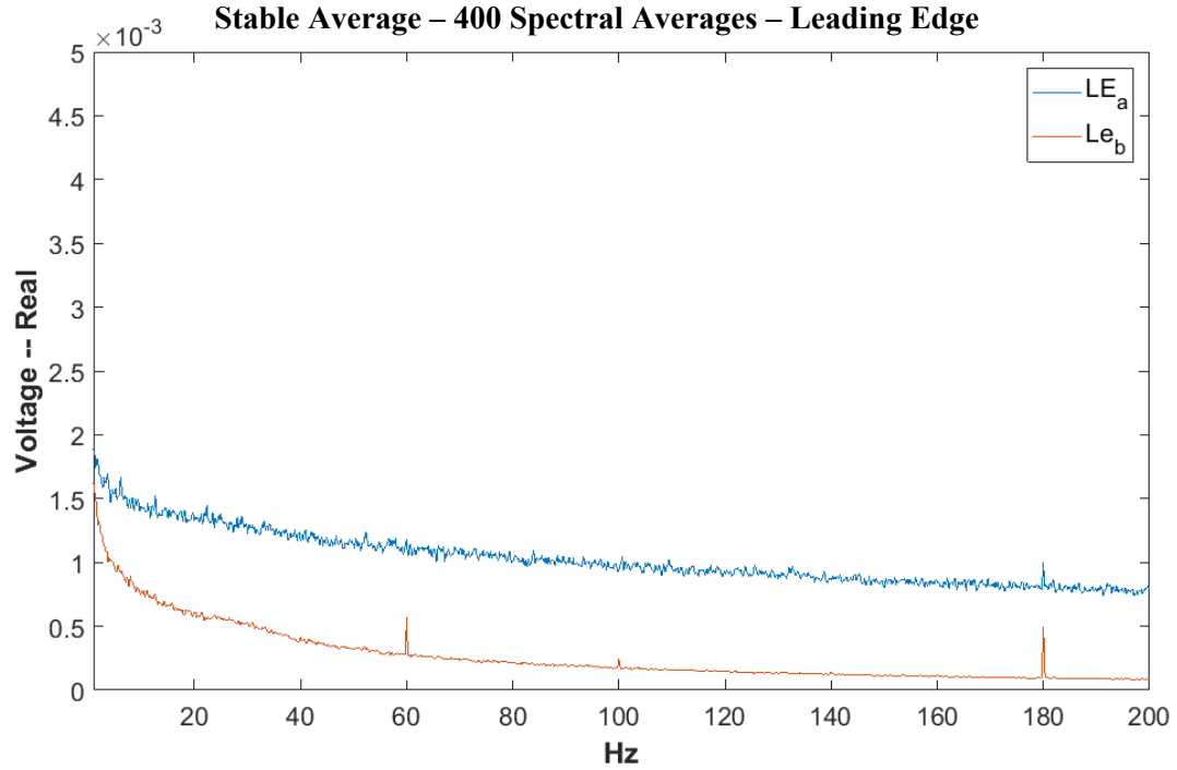
Figure 90. Leading Edge Hot-film PSD, 400 Averages, 0-.005V v. 0-200 Hz
