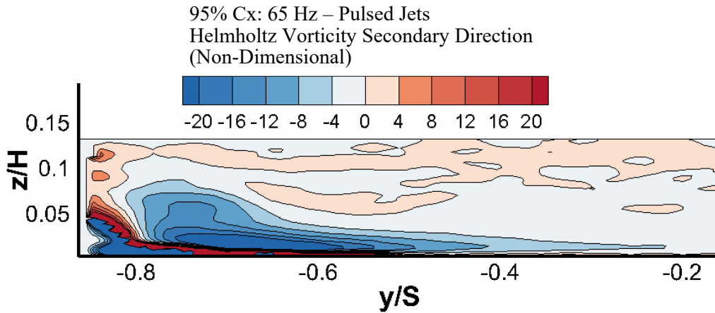
Figure 174. Helmholtz Secondary Vorticity - 65 Hz Pulsed Jets 95% Cx
