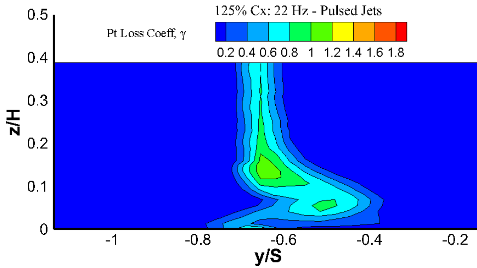
Figure 107. 22 Hz Pulsed Jets 125% C x Total Pressure Loss Map
