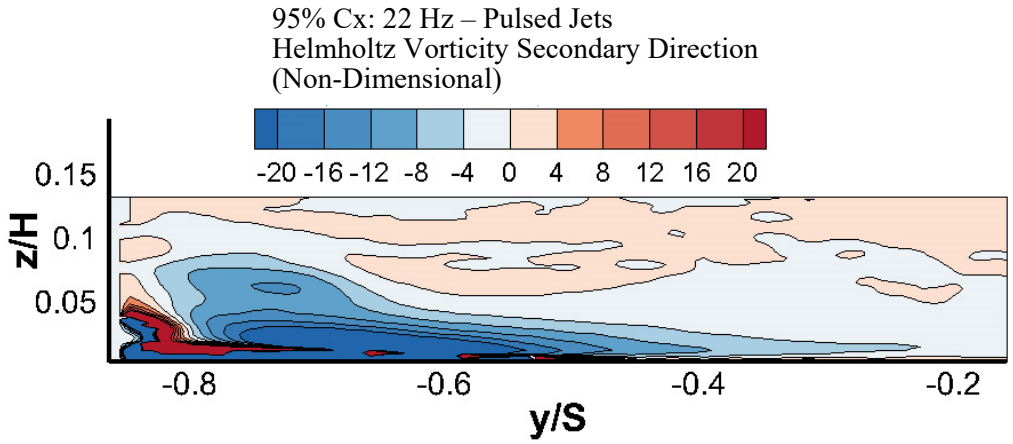
Figure 171. Helmholtz Secondary Vorticity - 22 Hz Pulsed Jets 95% Cx
