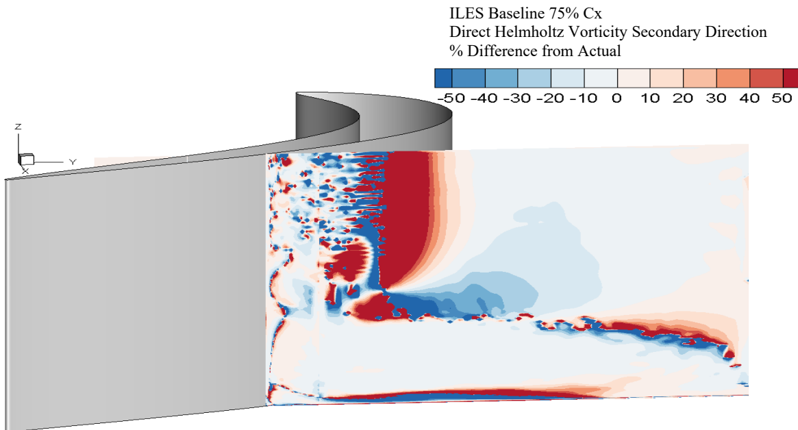
Figure 154. ILES Baseline, Comparison of Actual to Direct Helmholtz Secondary
