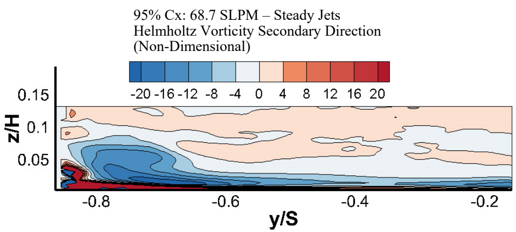
Figure 180. Helmholtz Secondary Vorticity - 68.7 SLPM Steady Jets 95% Cx
