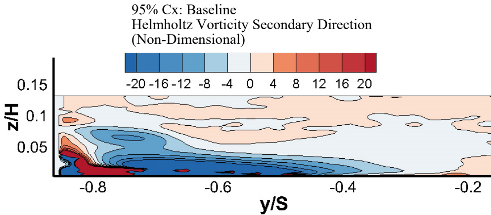
Figure 168. Helmholtz Secondary Vorticity - Baseline 95% Cx
