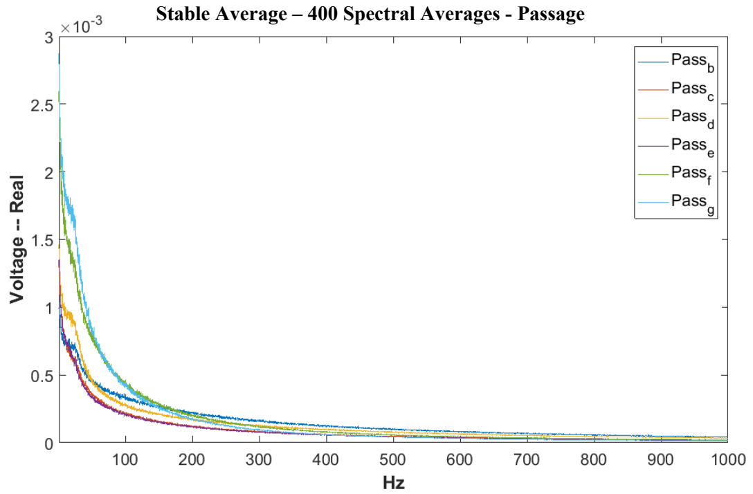
Figure 83. In-Passage Hot-film PSD, 400 Averages, 0-.003V v. 0-1000 Hz
