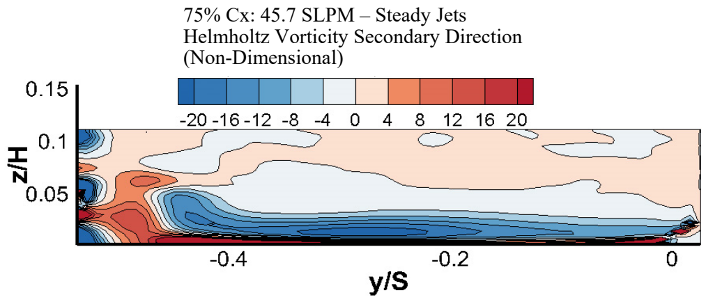
Figure 179. Helmholtz Secondary Vorticity - 45.7 SLPM Steady Jets 75% Cx
